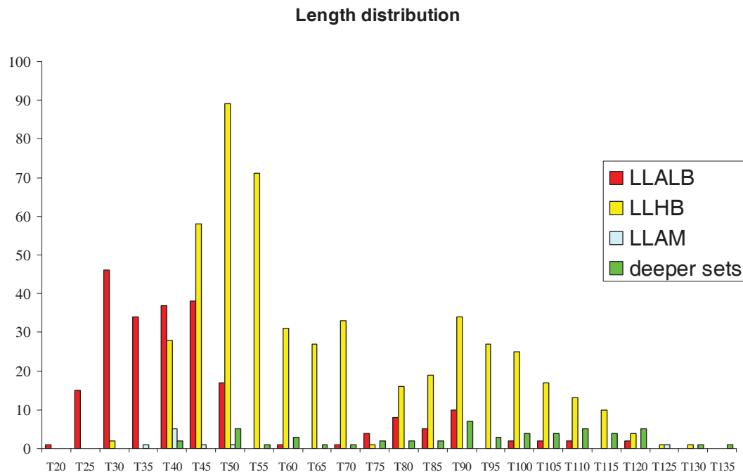
Figure 3. Length distribution per boat strata and gear type. Exist significative differences between boat strata length distribution (chi-squared= 1521.42; df= 69; P < 0.0001 ).
